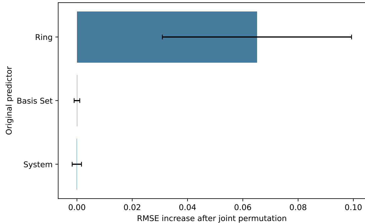
Grouped permutation importance: norm, |Q_2|(0)
